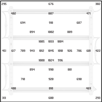
4 BAR | 800W | AVG PPFD: 754 5' FOOTPRINT | TESTED AT 24"
