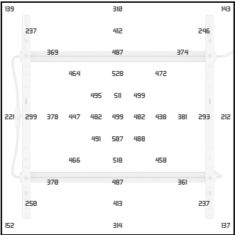
2 BAR | 400W | AVG PPFD: 377 5' FOOTPRINT | TESTED AT 24"
