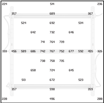
3 BAR | 600W | AVG PPFD: 558 5' FOOTPRINT | TESTED AT 24"
