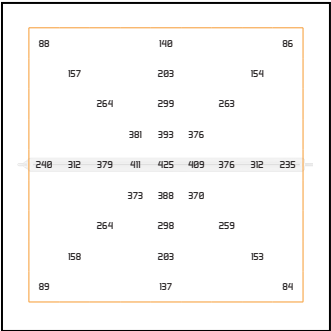
1 BAR | 200W | AVG PPFD: 263 4' FOOTPRINT | TESTED AT 24"
